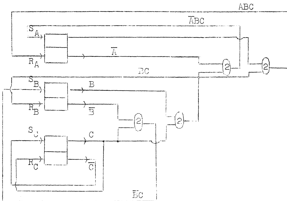
fig.7 3-bits teller
